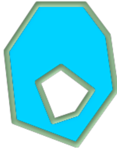
polygon holes with boundary multilinestring
