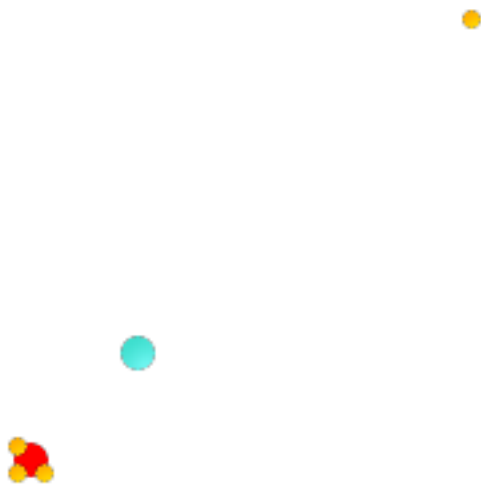
Comparison of the centroid (turquoise point) and geometric median (red point) of a four-point MultiPoint (yellow points).
